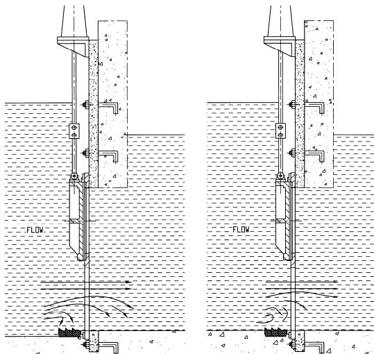
Rubbish Blocking Problem
