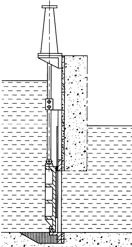
Flash Bottom Mounted Method
